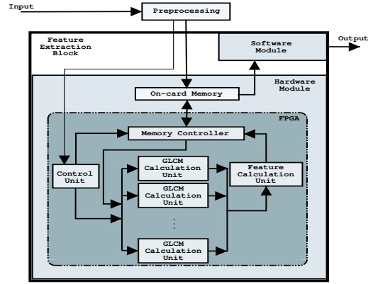
Figure 1. Overview of the architecture
